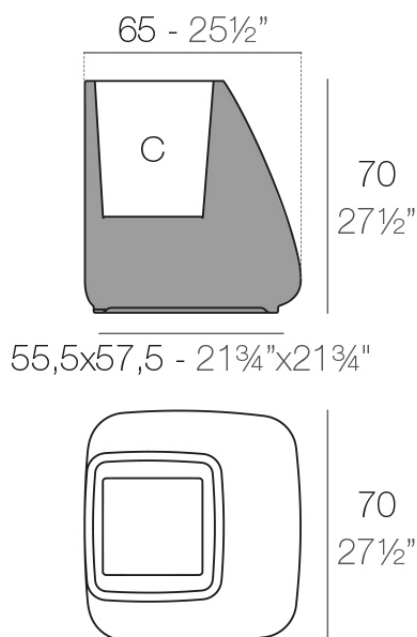
Macetero Medium Medium Planter
